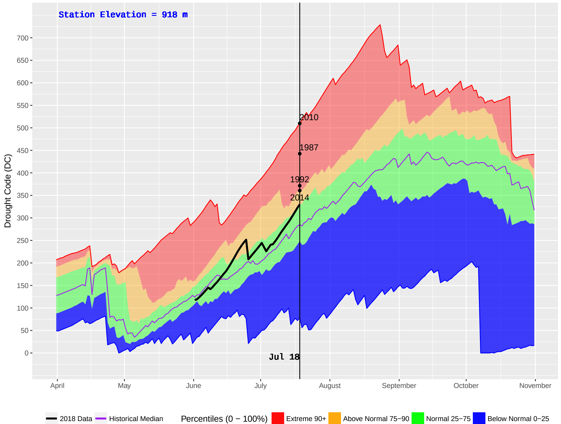
AUGIER LAKE (167) : Historical (1984–2016) and Current (2018) Daily Drought Code (DC)
