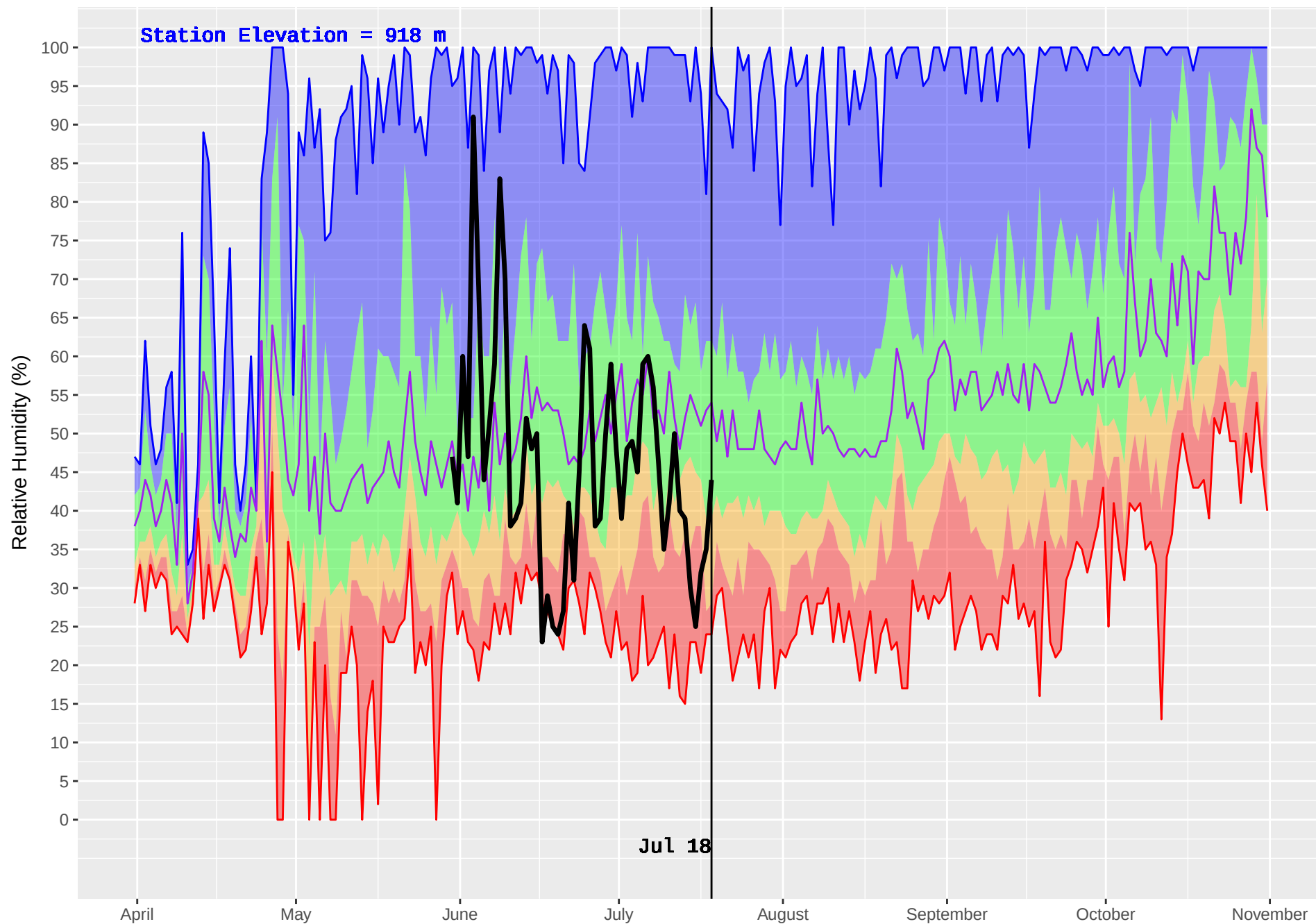
AUGIER LAKE (167) : Historical (1984–2016) and Current (2018) Daily Relative Humidity
