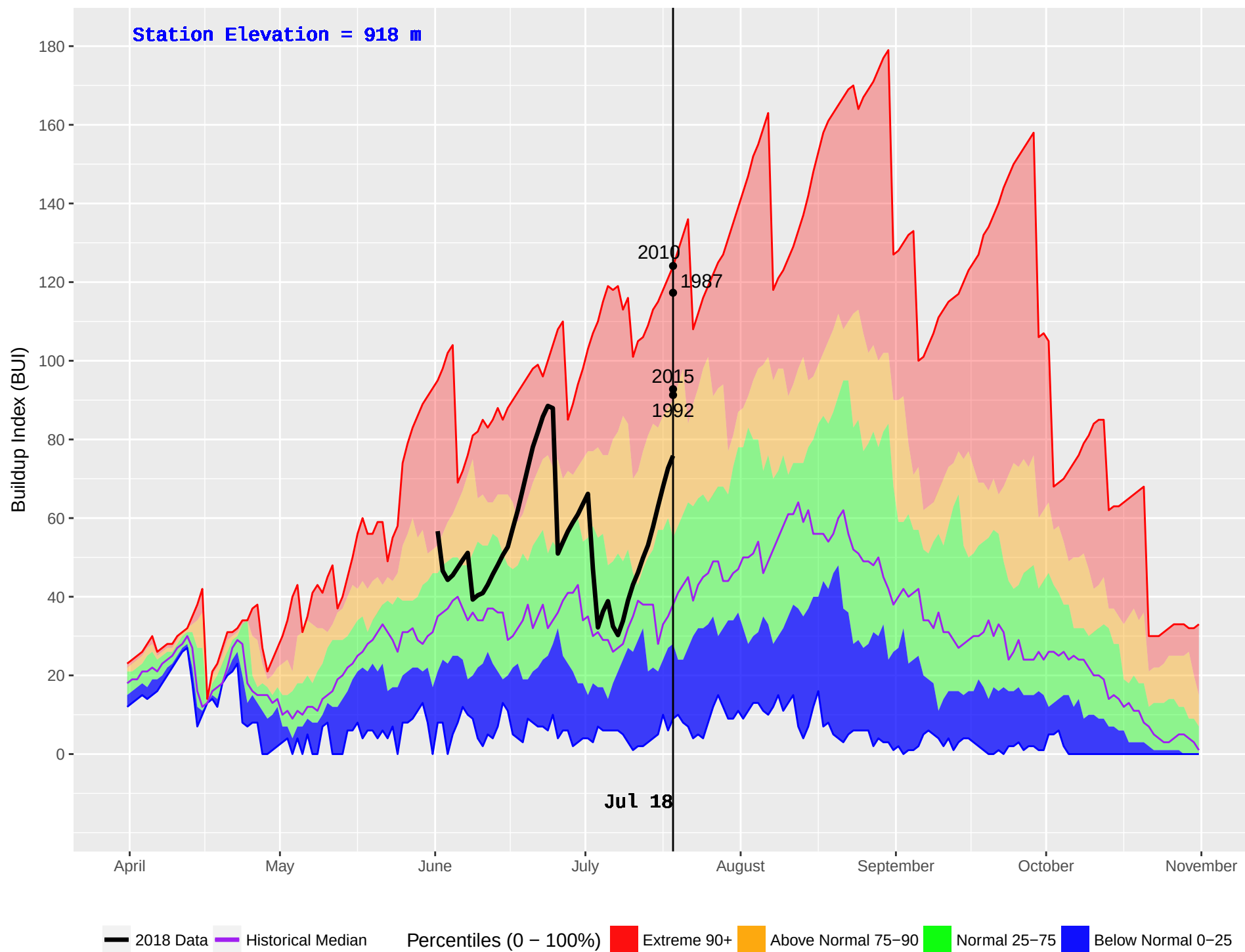
AUGIER LAKE (167) : Historical (1984–2016) and Current (2018) Daily Buildup Index (BUI)
