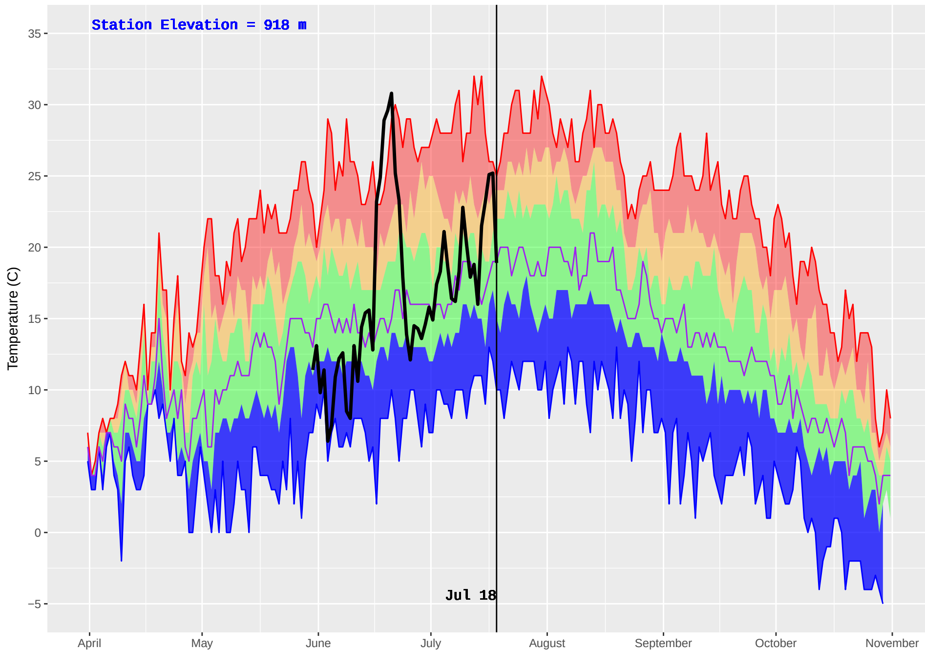
AUGIER LAKE (167) : Historical (1984–2016) and Current (2018) Daily Temperature
